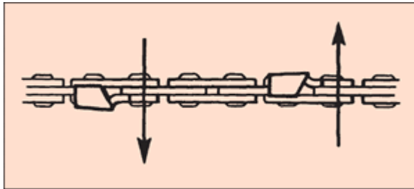
Fig 39: File from the inside of the cutter outwards.
